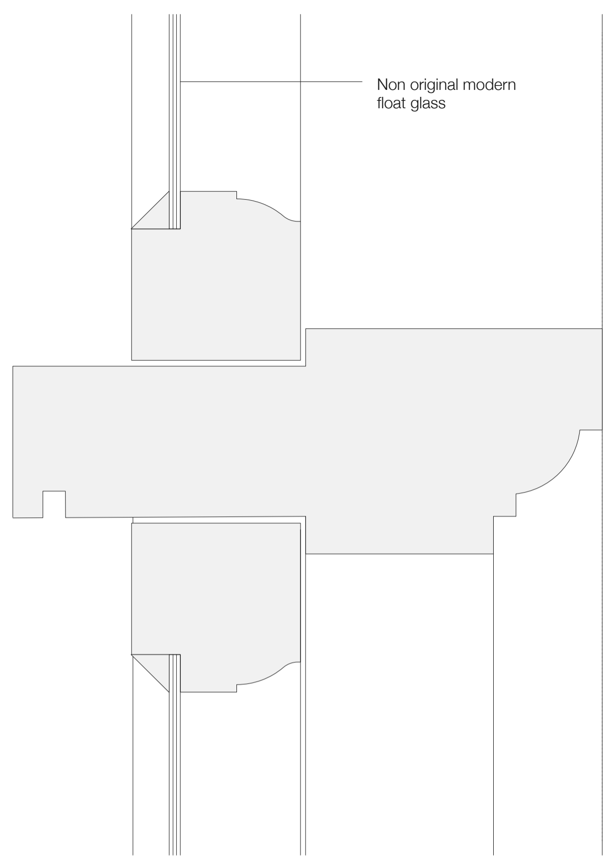
DETAIL A - THROUGH DOOR HEAD
