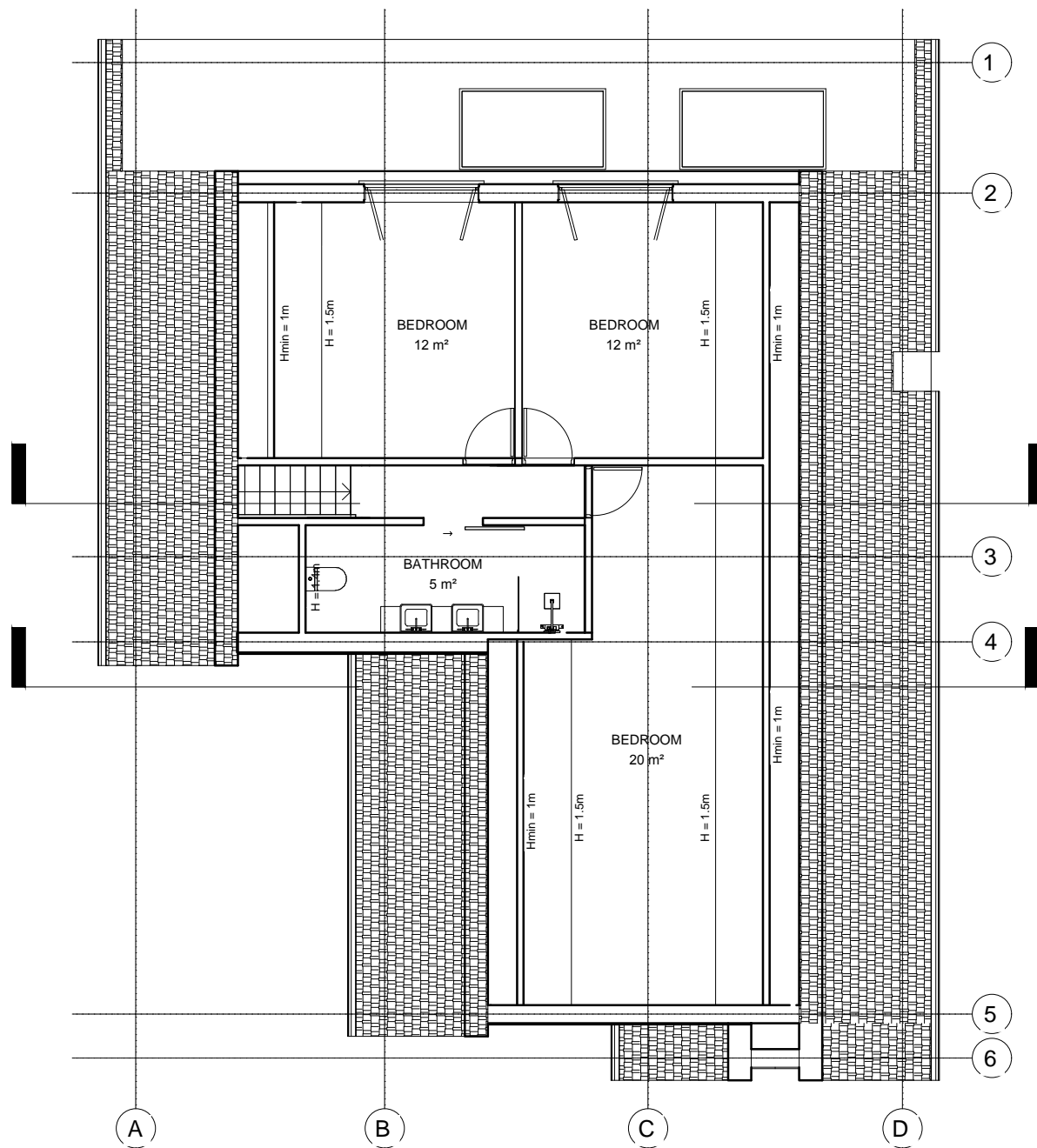
PROPOSED LOFT PLAN
