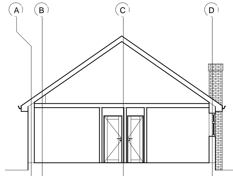
EXISTING SECTION
