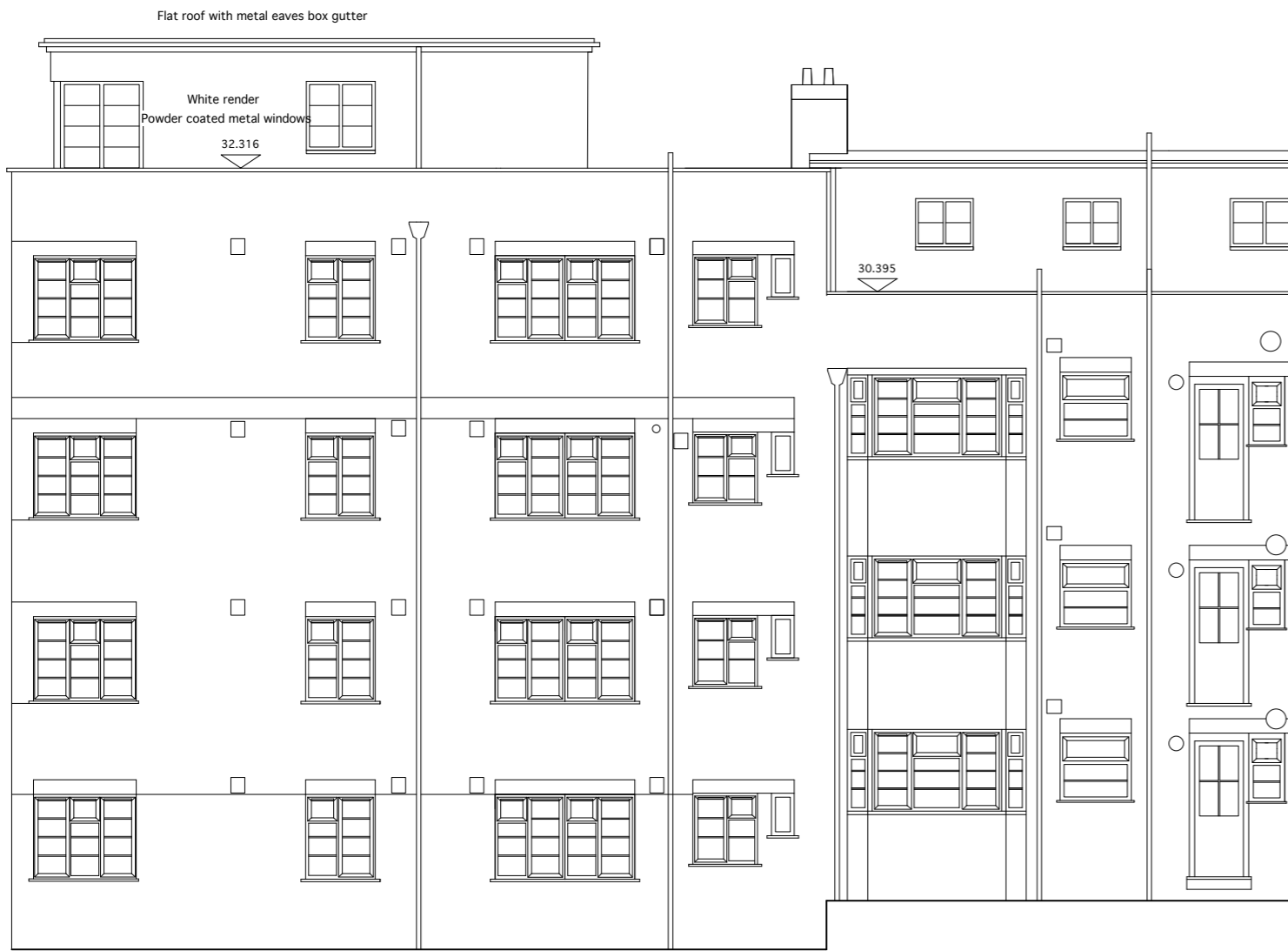
SOUTH ELEVATION
