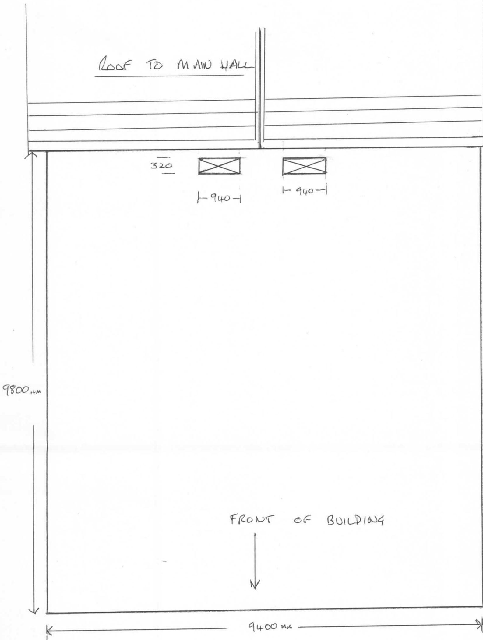
PLAN VIEW OF KITCHEN ROOF
