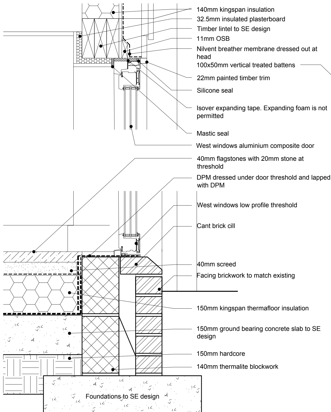
Detail E Door Threshold 1:5
