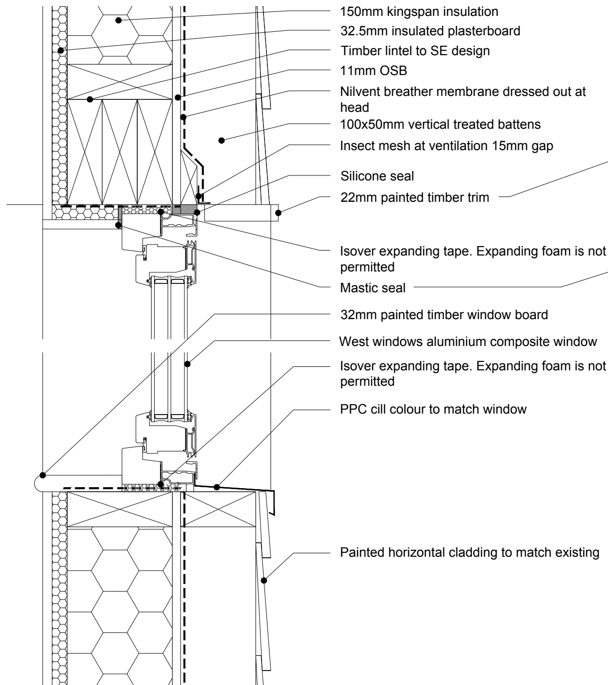
Detail B Cill & Head 1:5
