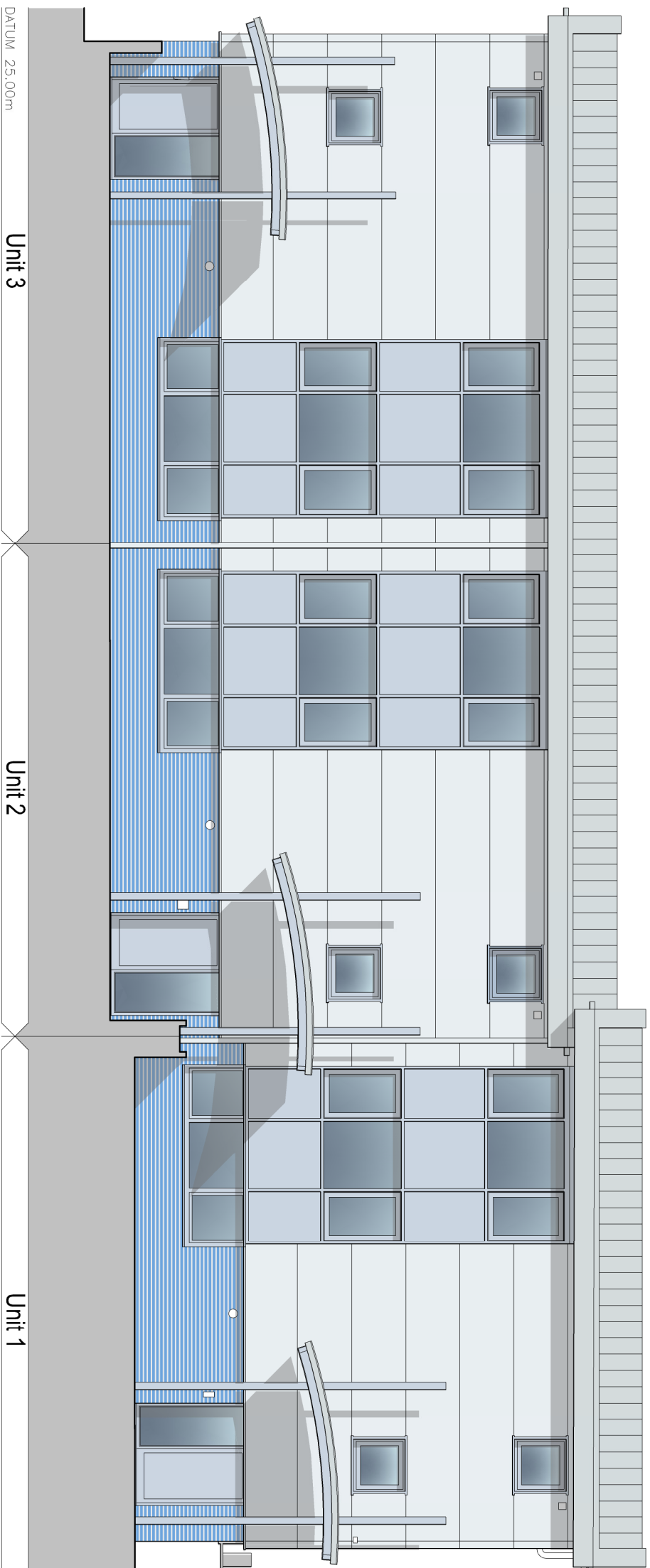
Existing north elevation Scale 1:100@A3
