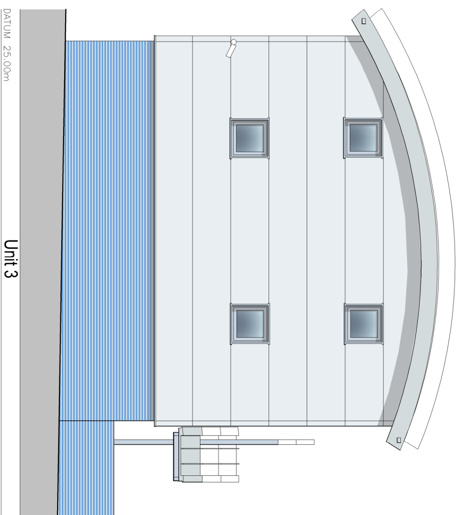
Existing east elevation Scale 1:100@A3 Profile of higher roof to unit 1 shown in the background
