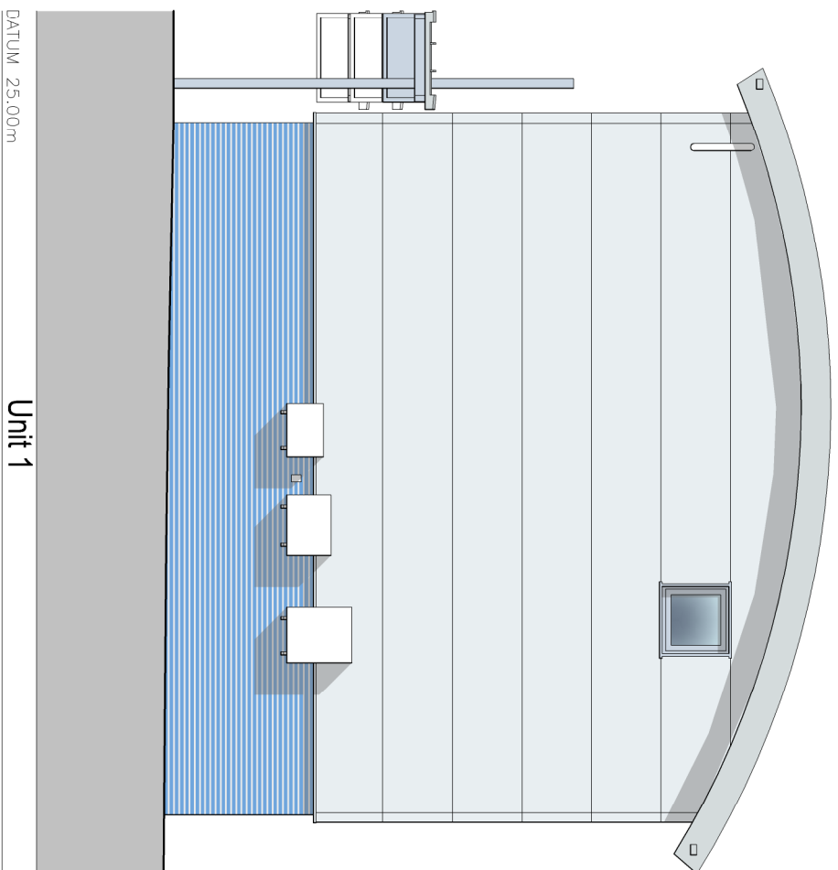
Existing west elevation Scale 1:100@A3
