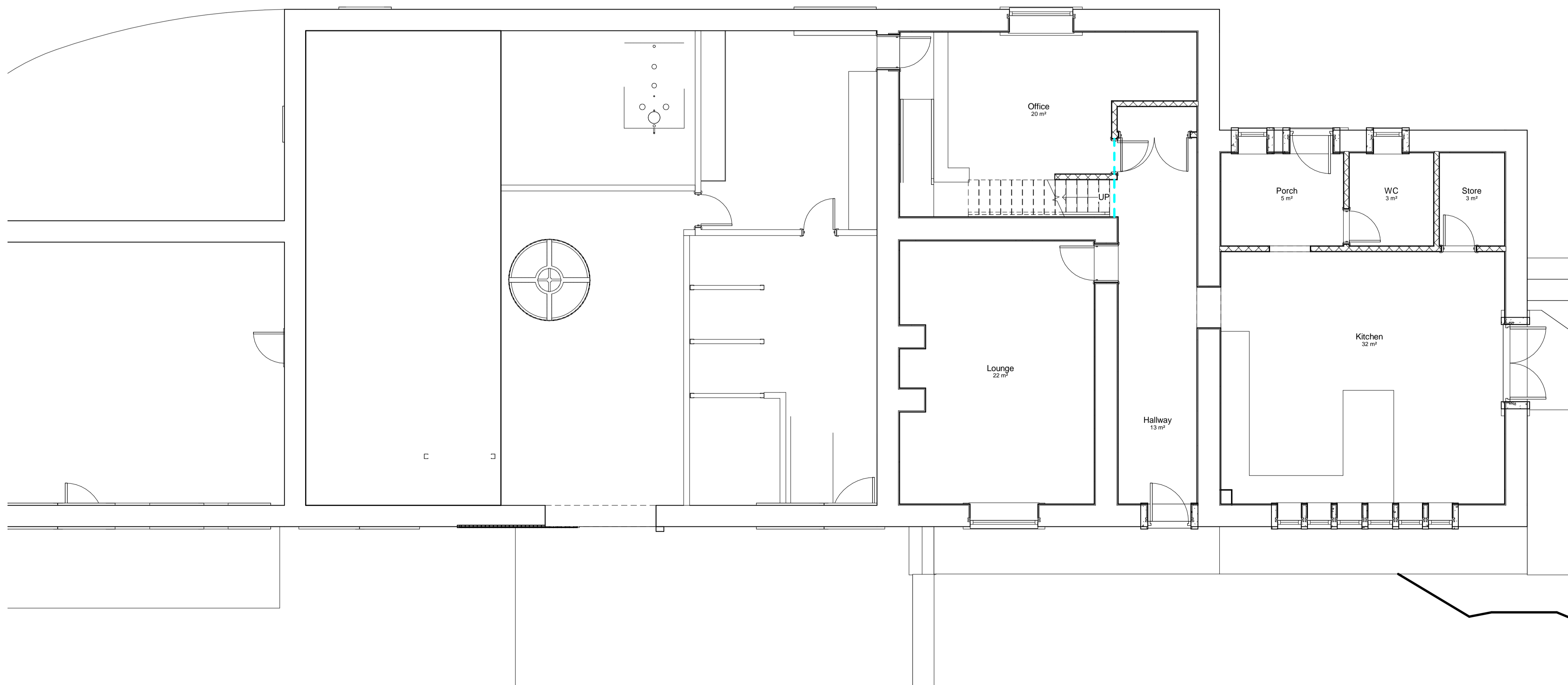
Ground Floor Plan Scale: 1 : 50
