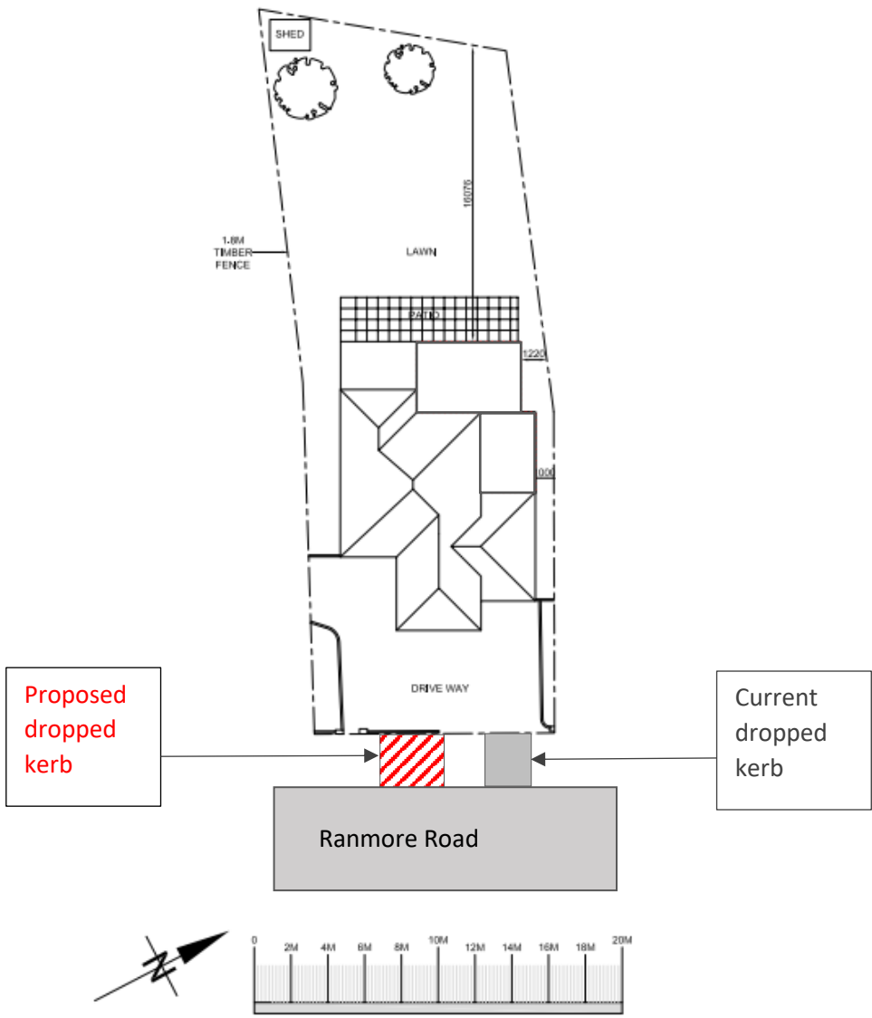
SCALE BAR 1:200 BLOCK PLAN
