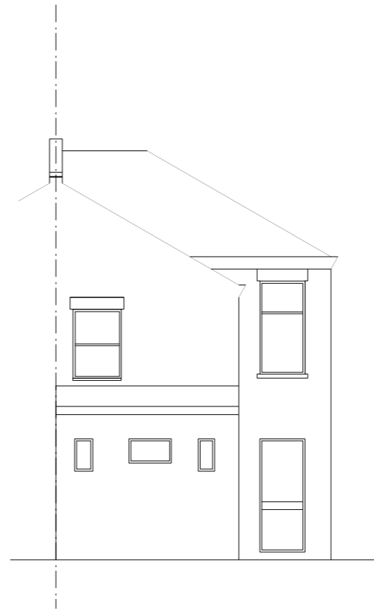
REAR ELEVATION
