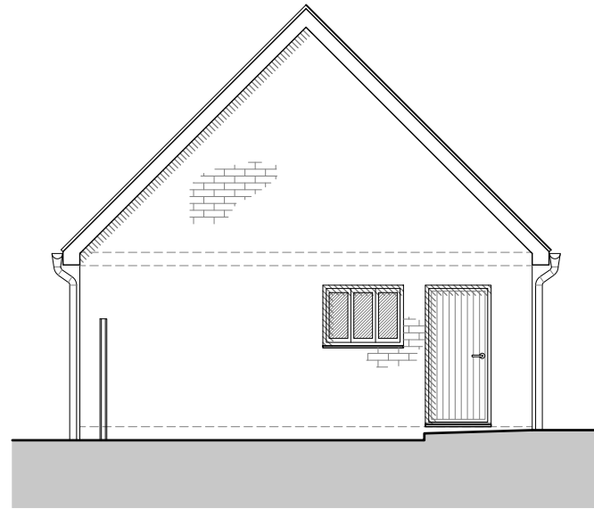
East Elevation
