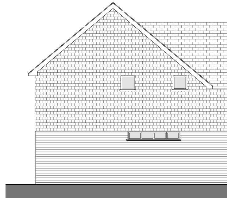
EXISTING NW ELEVATION(PART OF)
