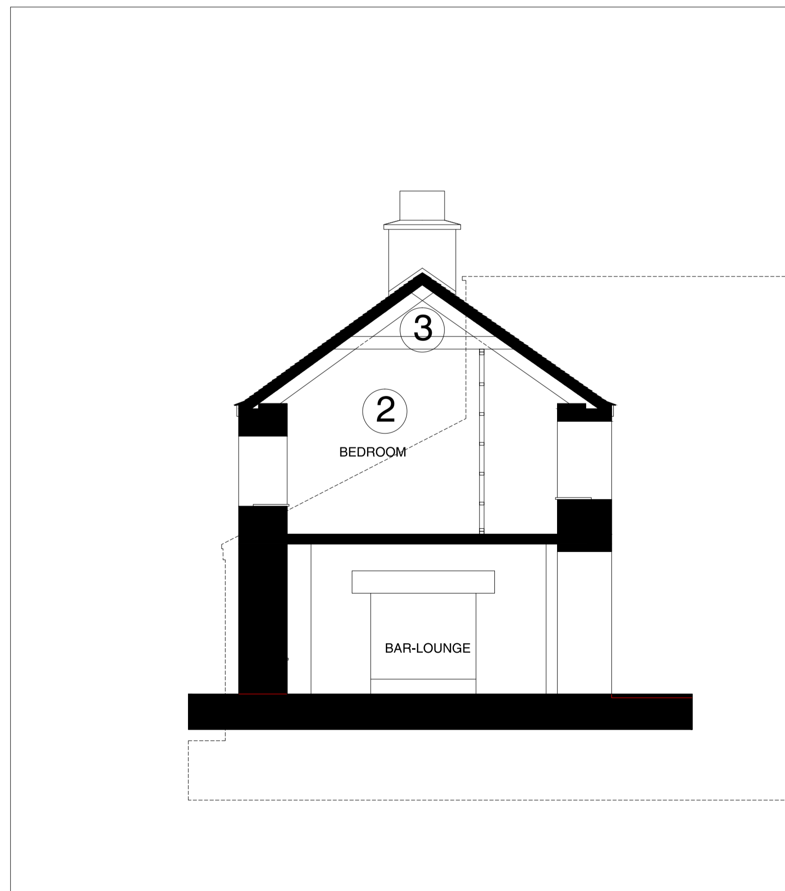
SECTION 4-4: THROUGH BAR-BLOCK 1:50@A1
