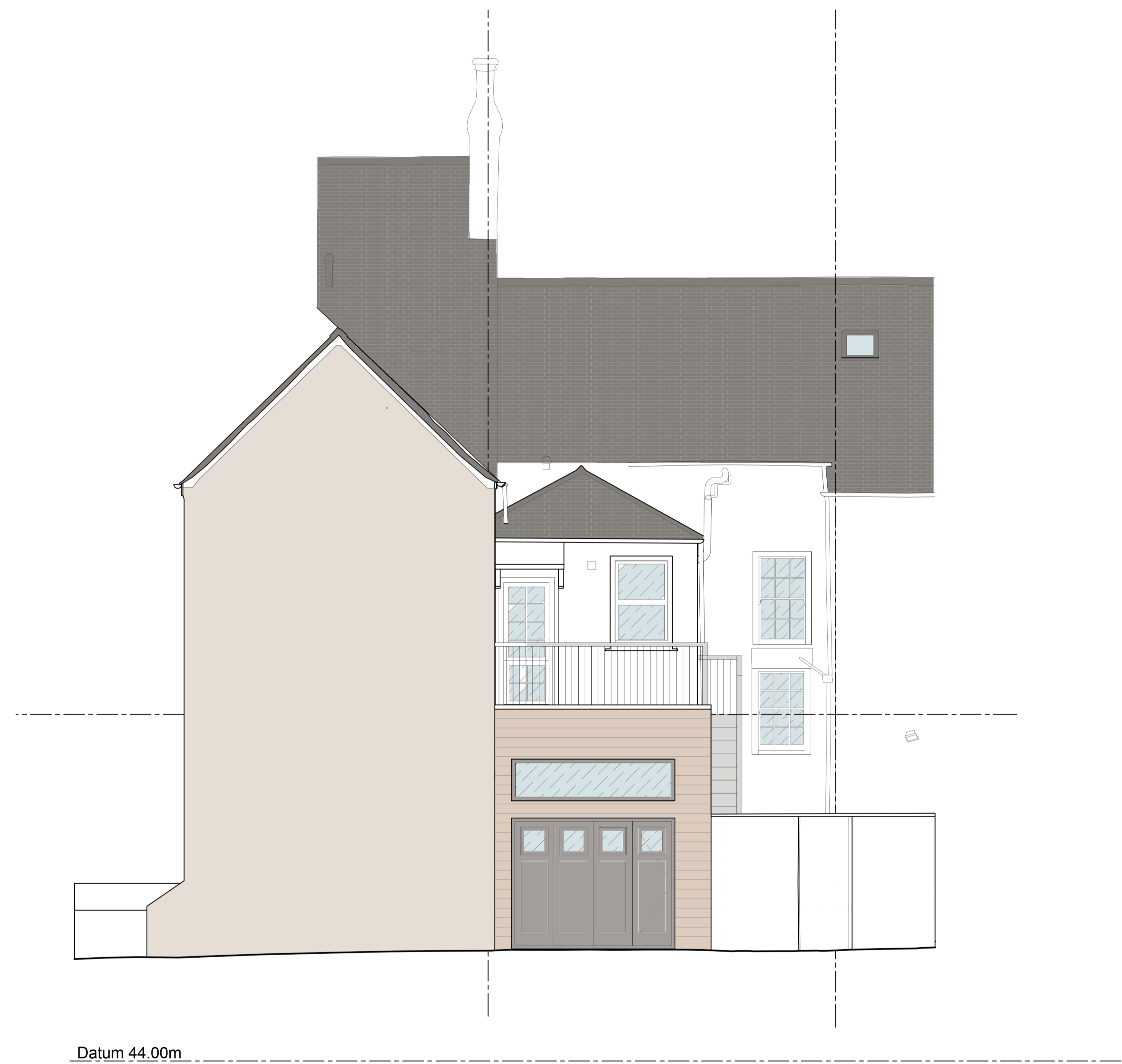
PROPOSED ELEVATION 3 Scale 1:50 @ A1
