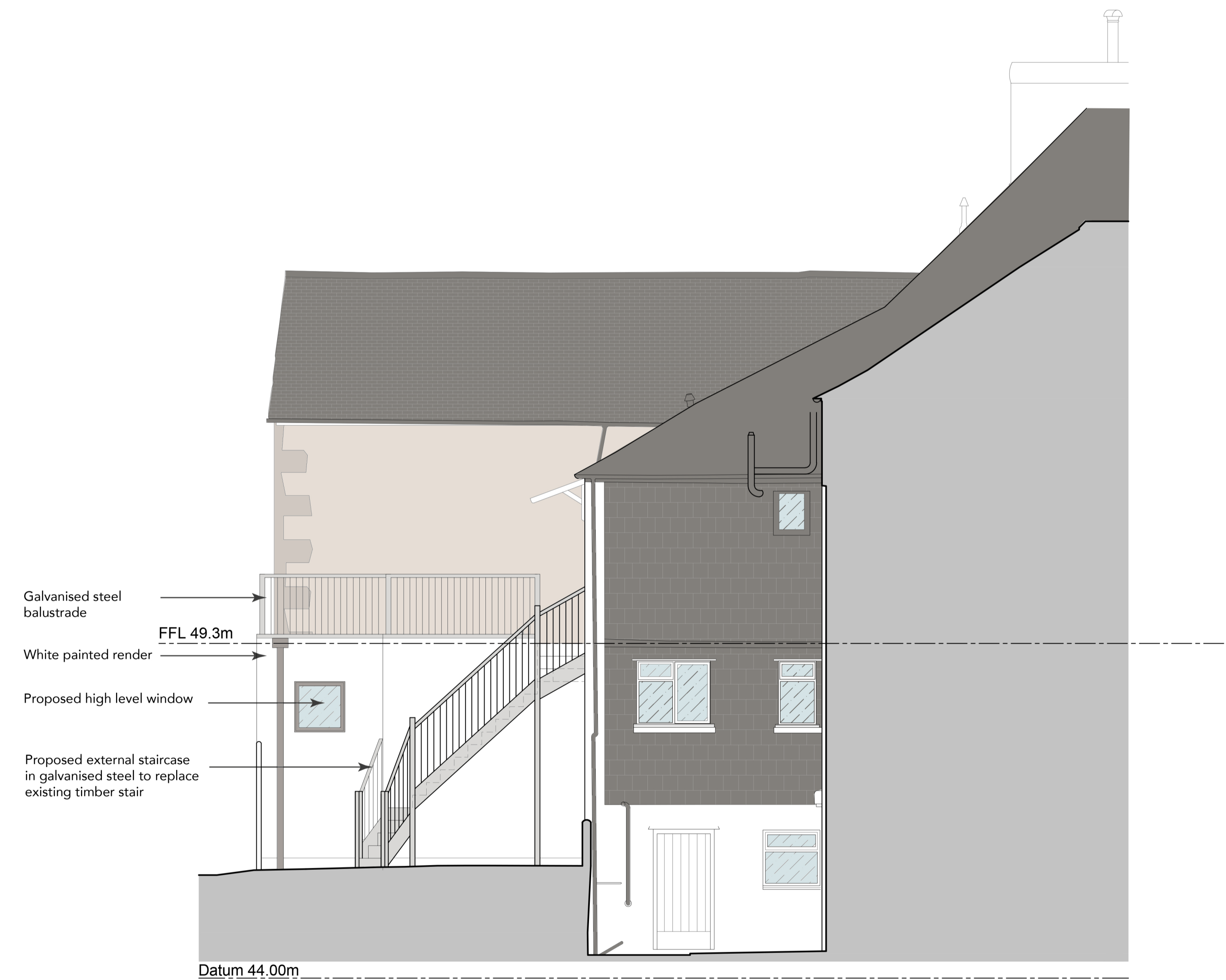
PROPOSED ELEVATION 4 Scale 1:50 @ A1
