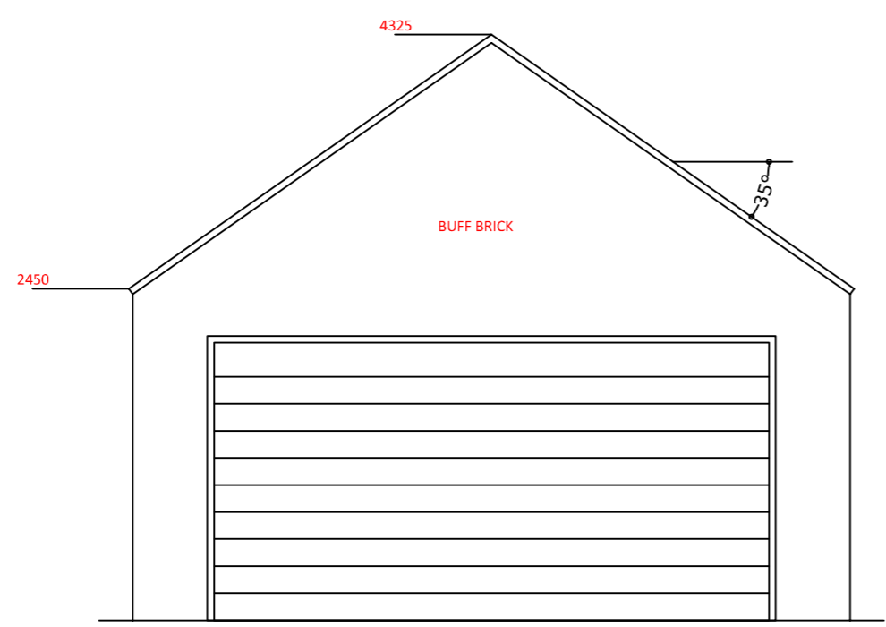
SOUTH ELEVATION
