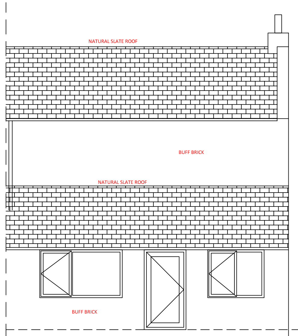
NORTH ELEVATION
