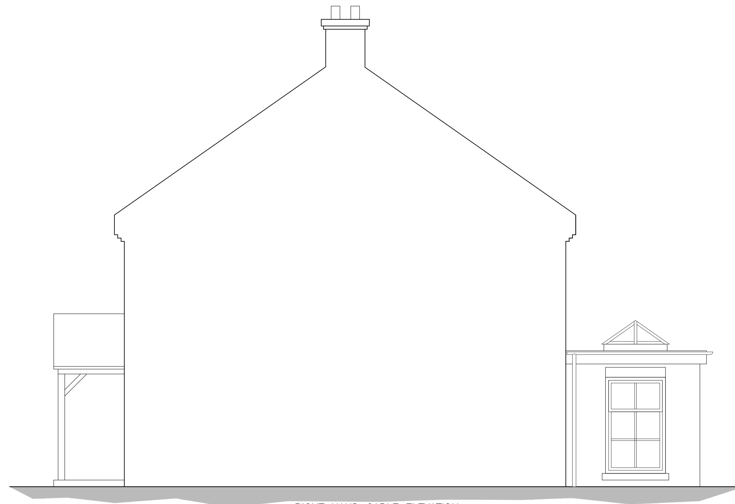
RIGHT HAND GABLE ELEVATION (1:50)
