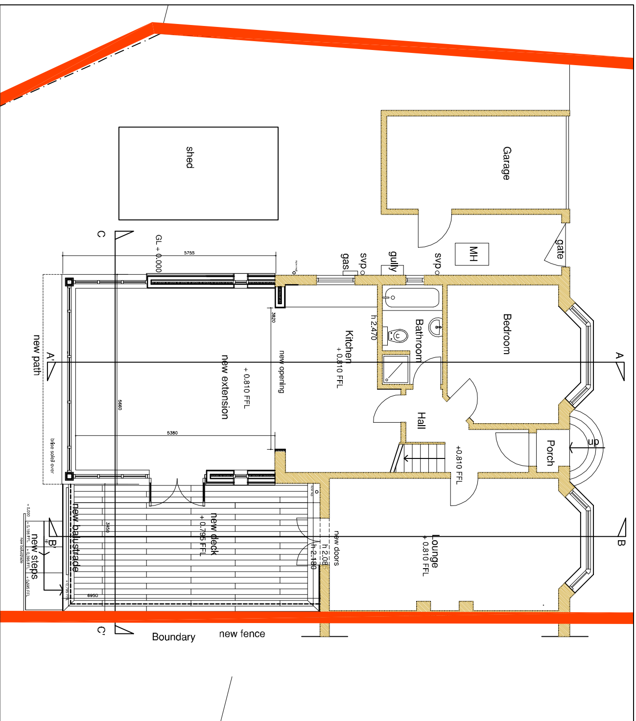
1:100 Ground Floor Plan as proposed
