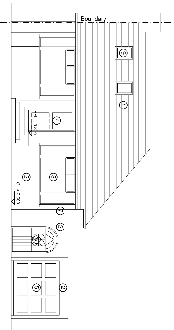
1:100 North Elevation as existing
