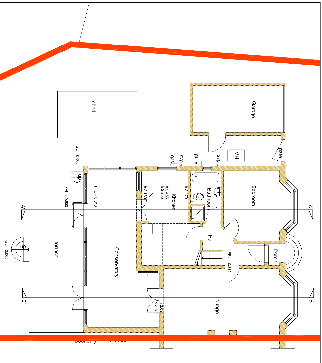
1:100 Ground Floor Plan as existing
