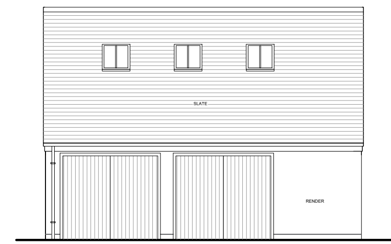
EAST ELEVATION (Front)
