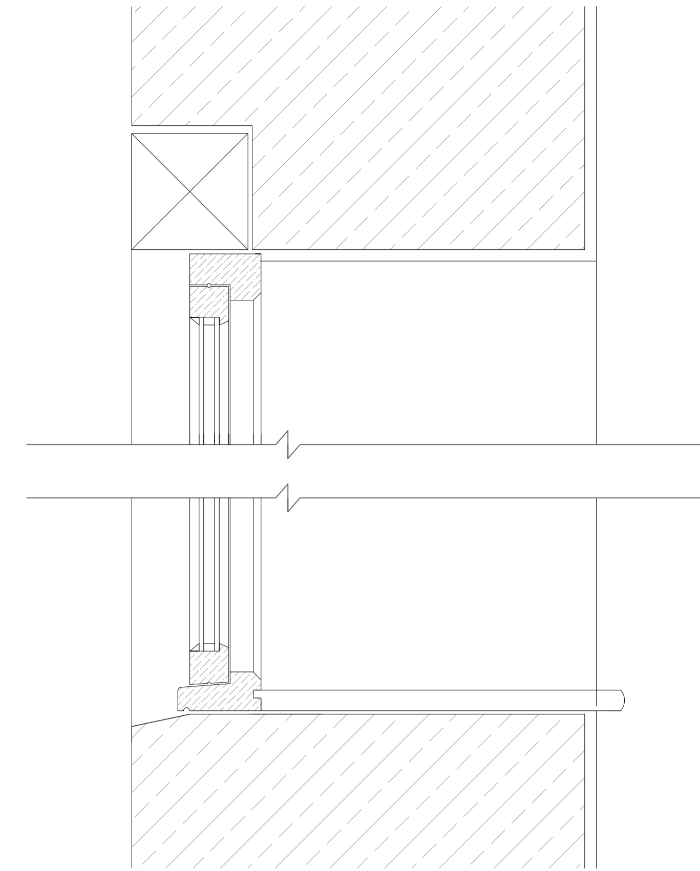
Vertical section through casement window
