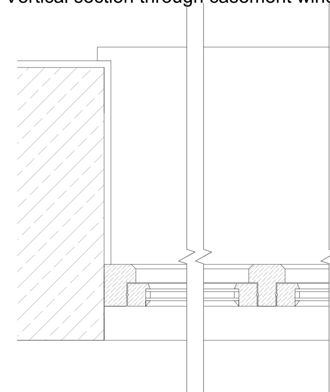
Vertical section through casement window
