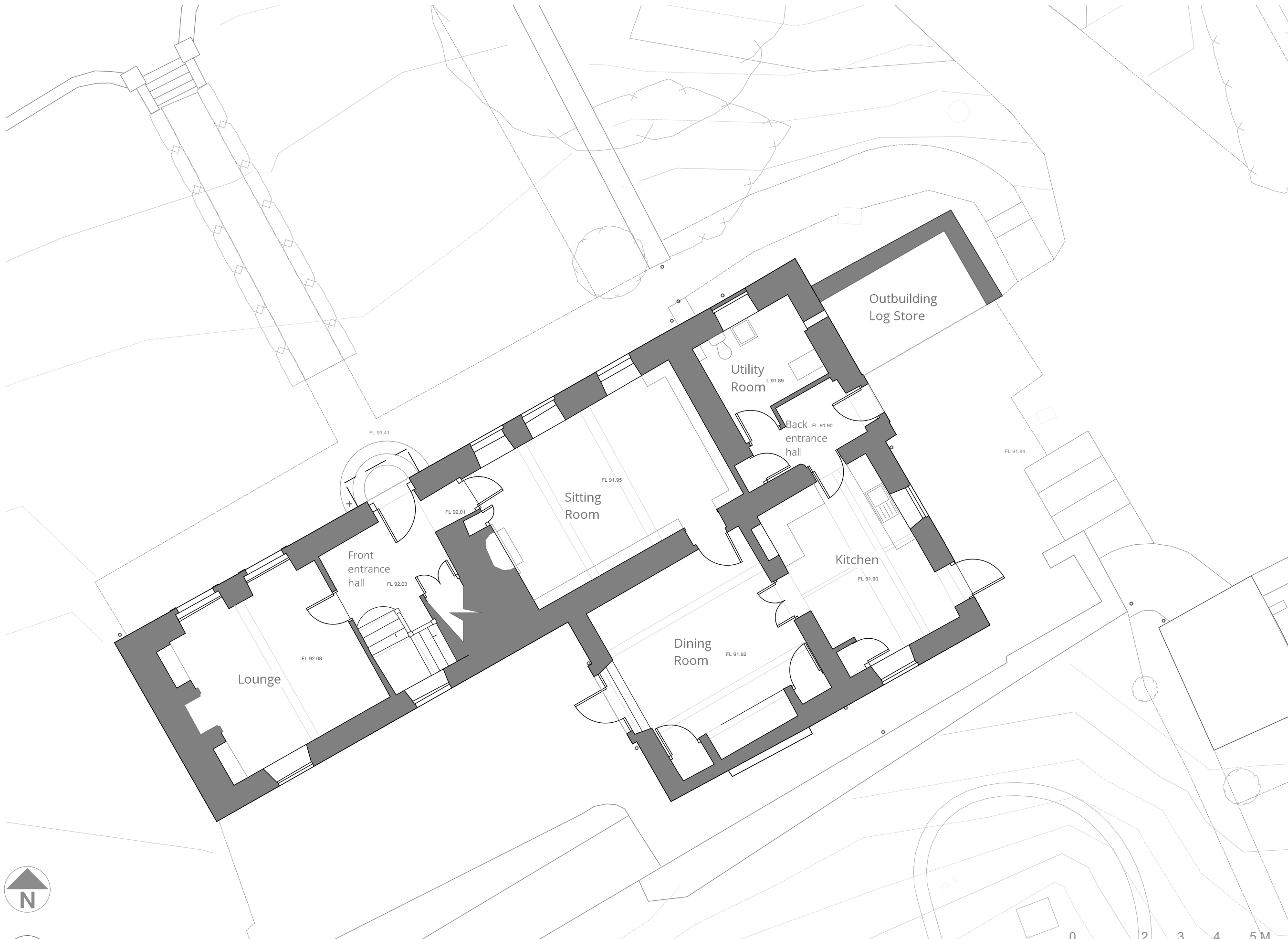
P/200 FARMHOUSE - EXISTING GROUND FLOOR PLAN 1:100
