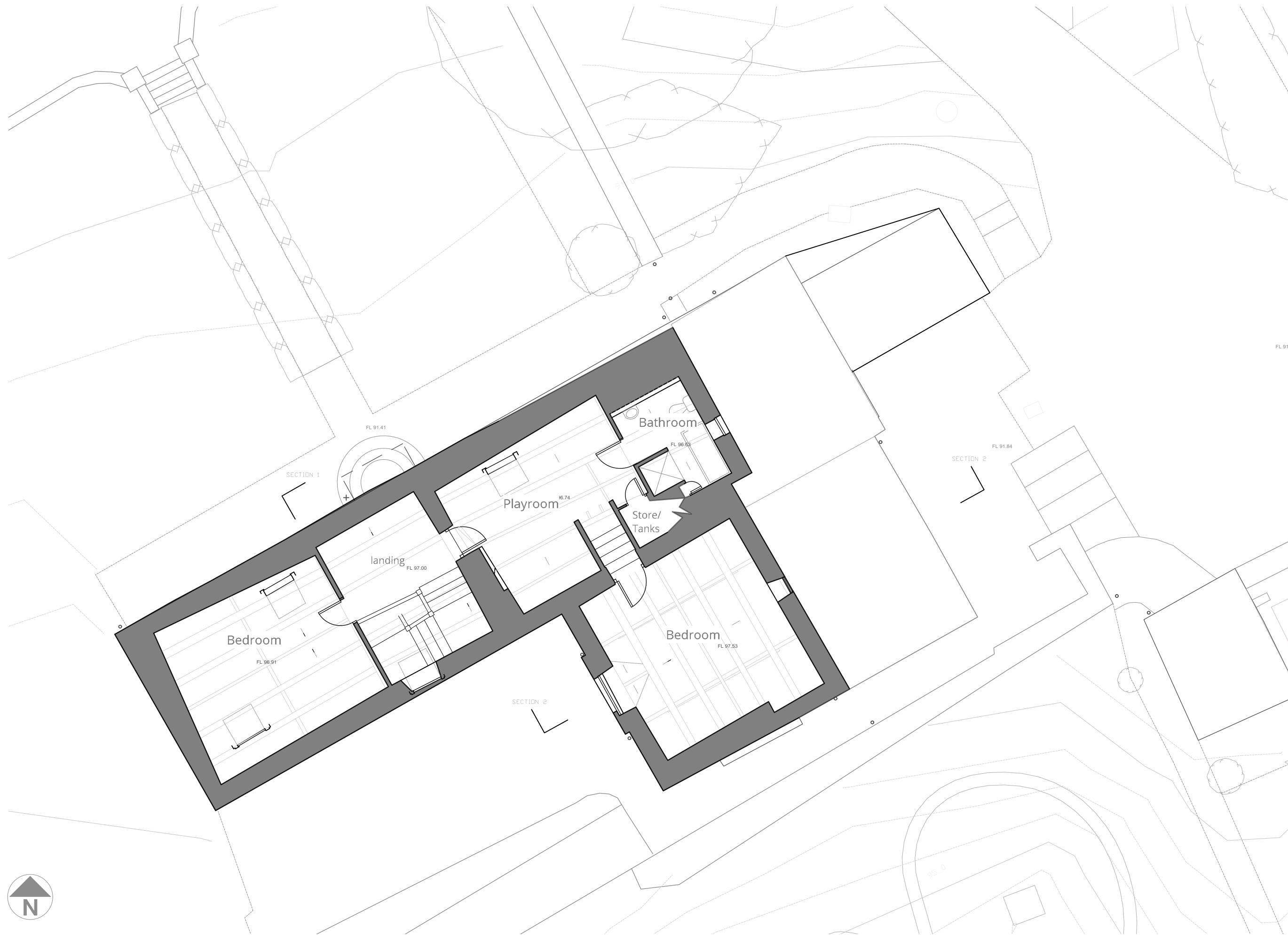
P/203 FARM HOUSE - EXISTING SECOND FLOOR PLAN 1:100
