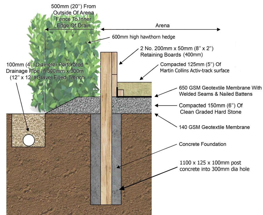
Arena fencing - 1:20
