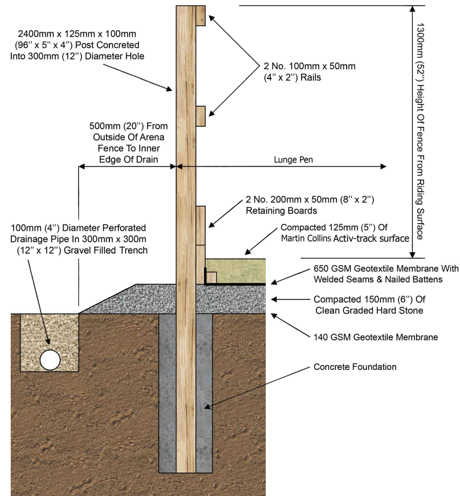
Lunge pen fencing - 1:20
