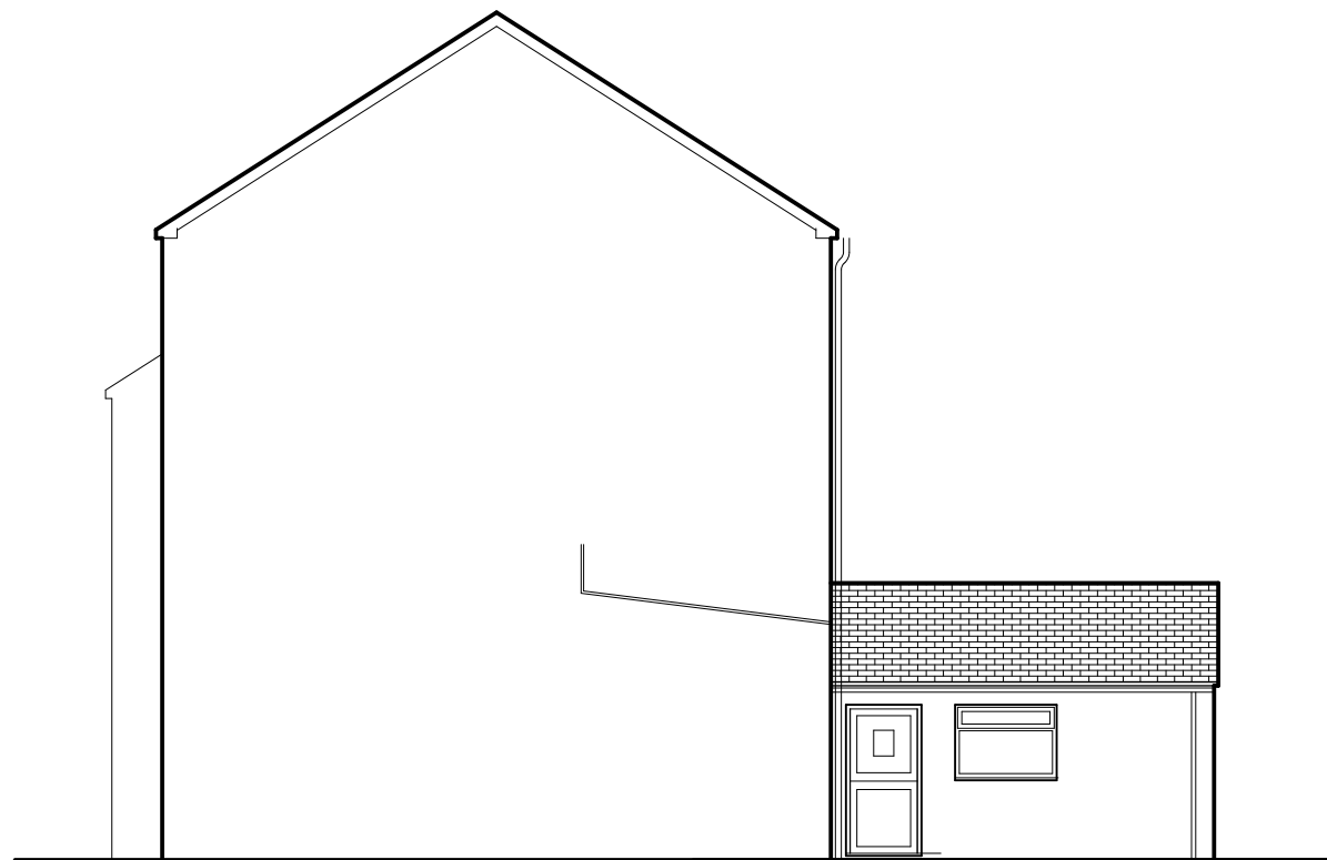
Side (North) Elevation
