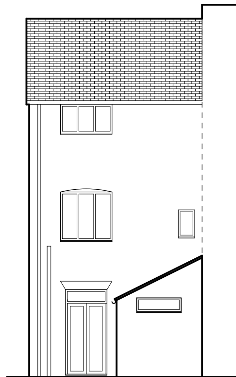
Rear (West) Elevation
