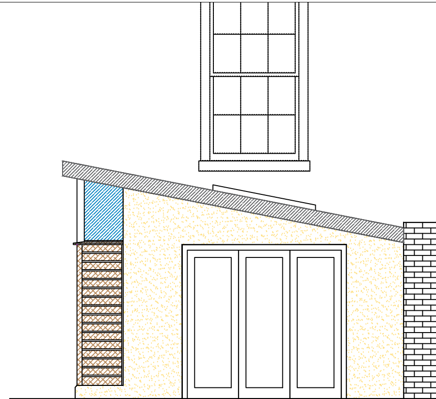
Rear Elevation
