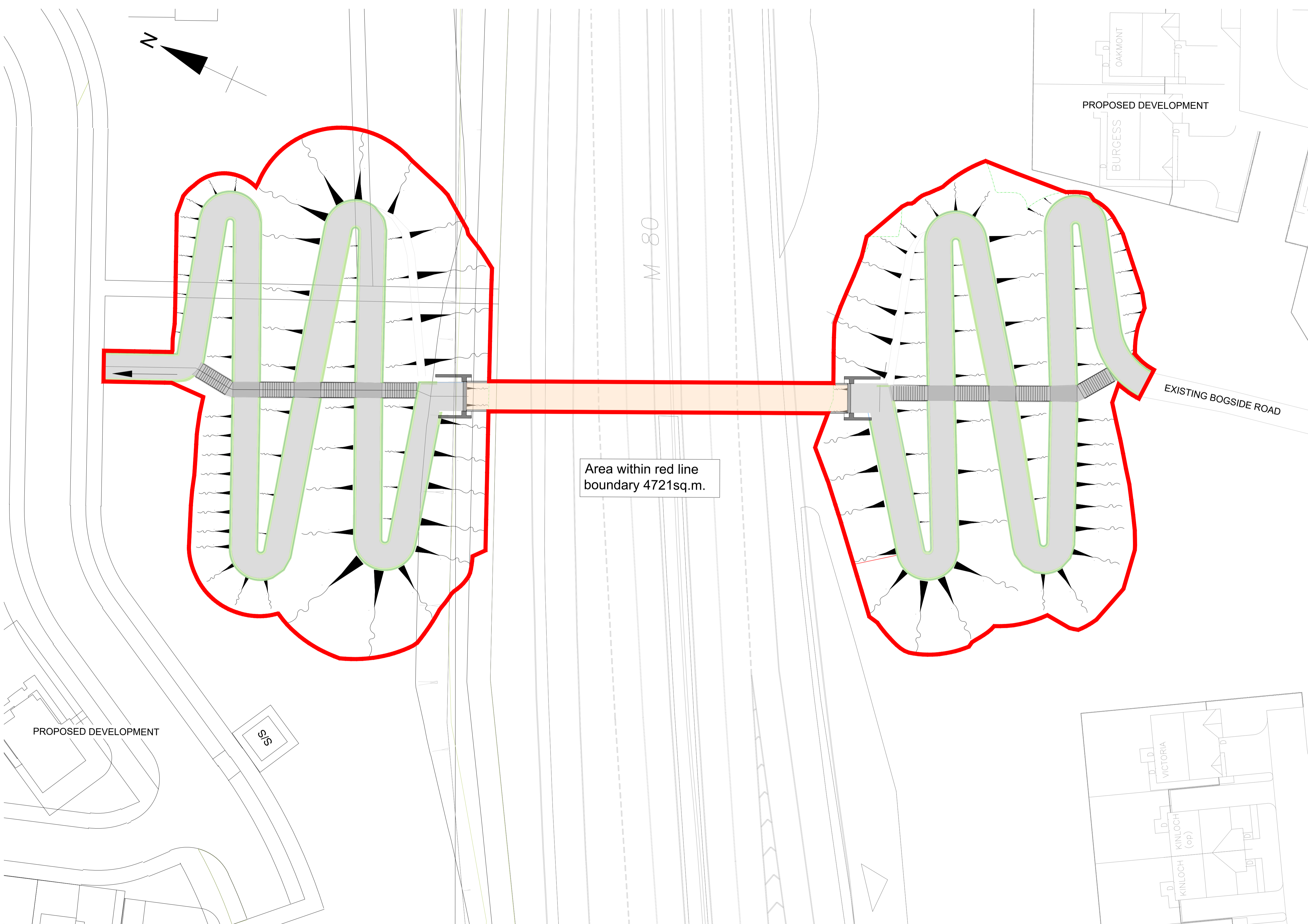
PROPOSED APPROACH RAMPS/STAIRS AND BRIDGE LAYOUT RED LINE BOUNDARY SCALE 1:250
