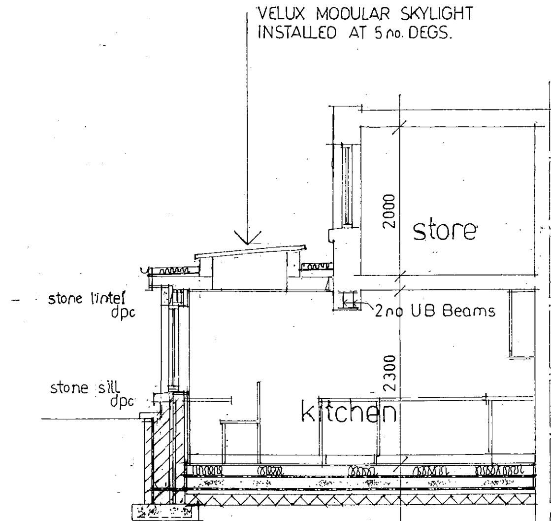
SECTION A A AS PROPOSED 1:50
