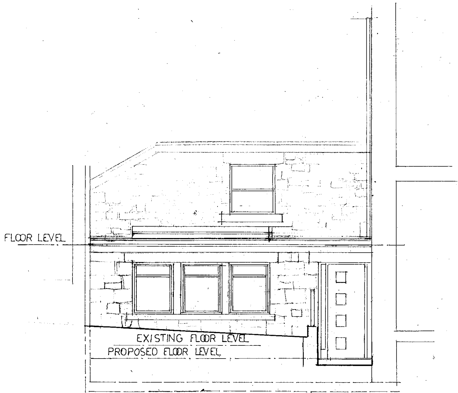
SOUTH EAST ELEVATION AS PROPOSED 1:50
