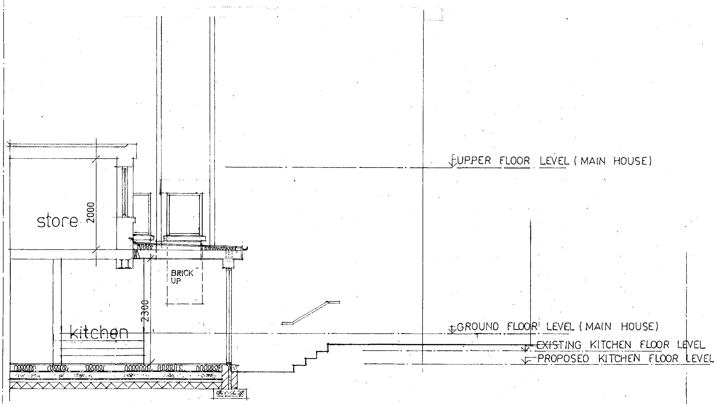
SECTION BB AS PROPOSED 1:50
