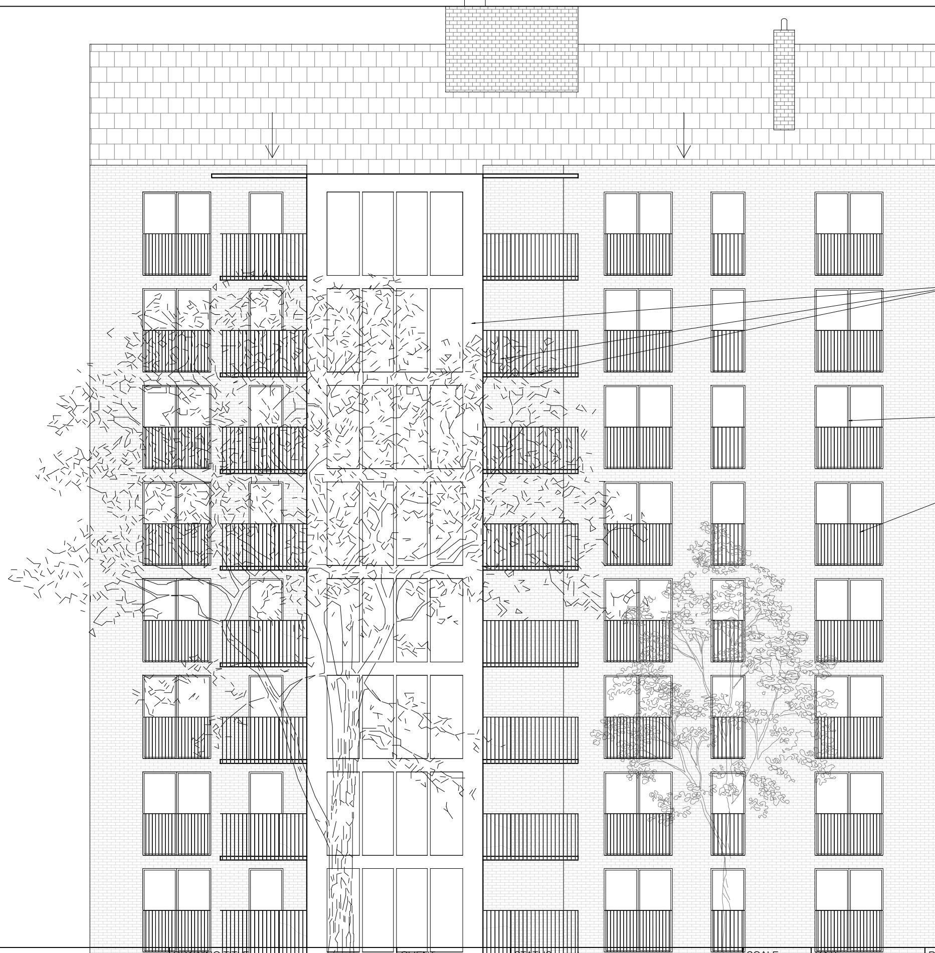
Proposed Front Elevation 1906-200
