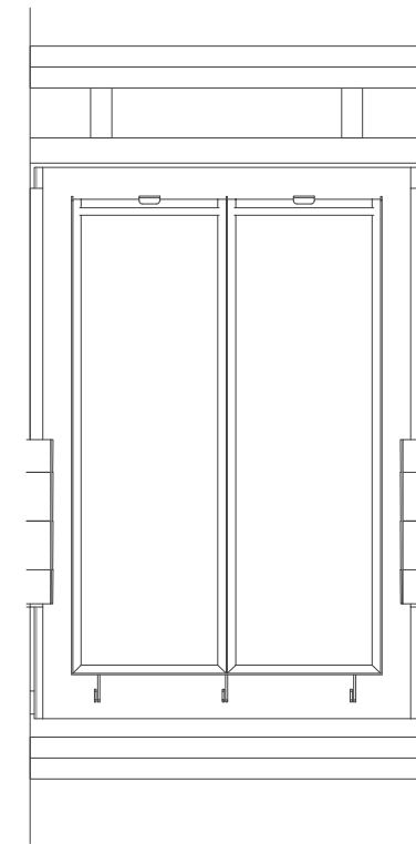
Proposed Conservation rooflight Elevation @ 1:20
