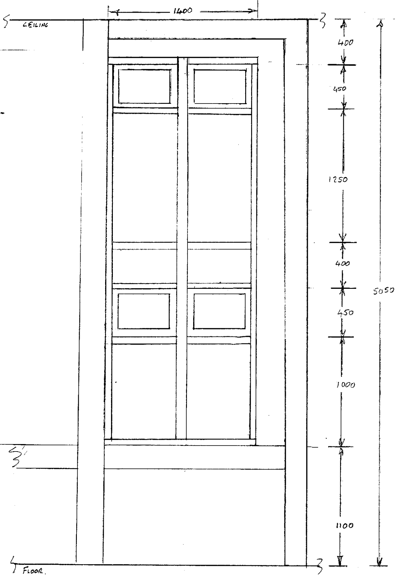
EXISTING WINDOW ELEVATION
