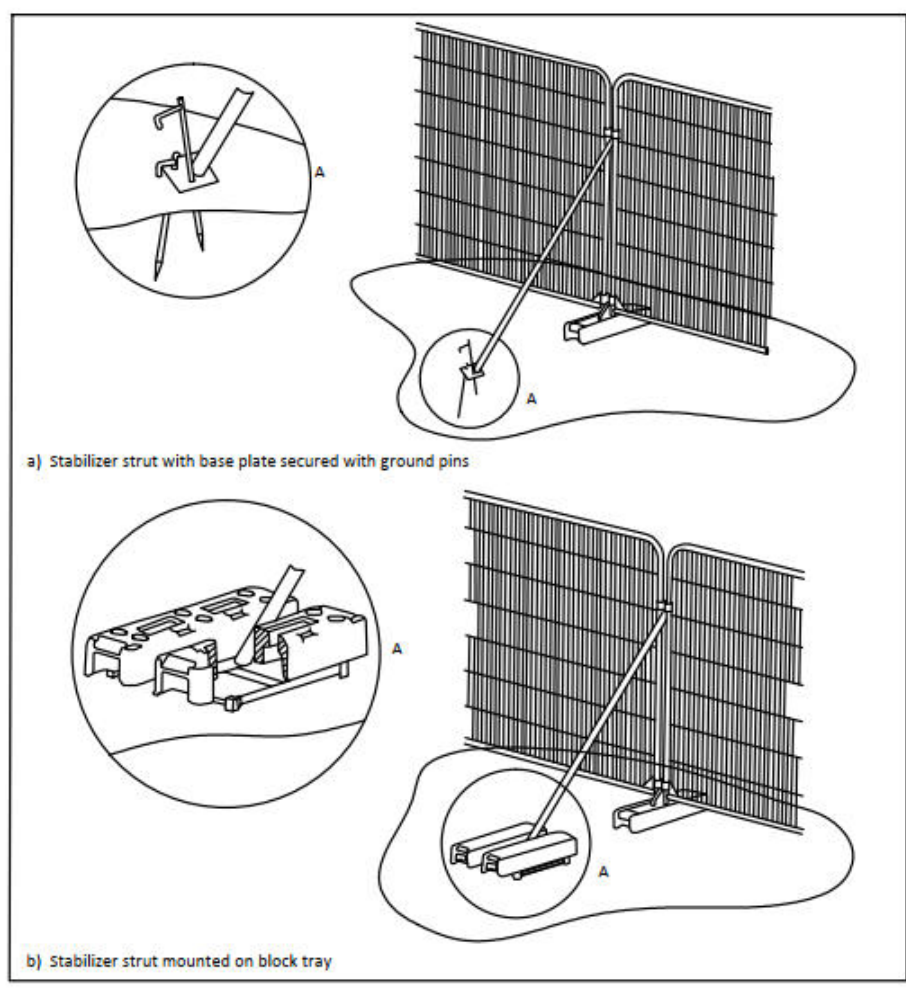
Figure 3 Examples of above-grounds stabilizing systems
