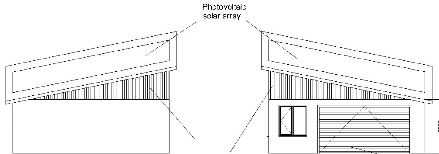
Proposed Garage SE Elevation
