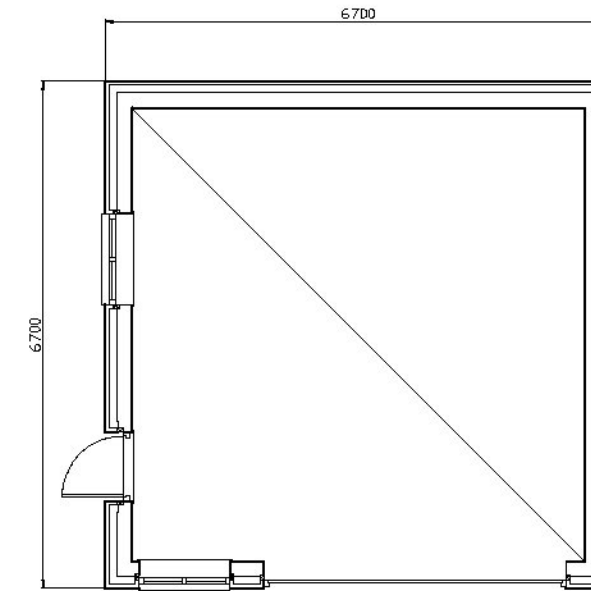
Proposed Garage Floor Plan
