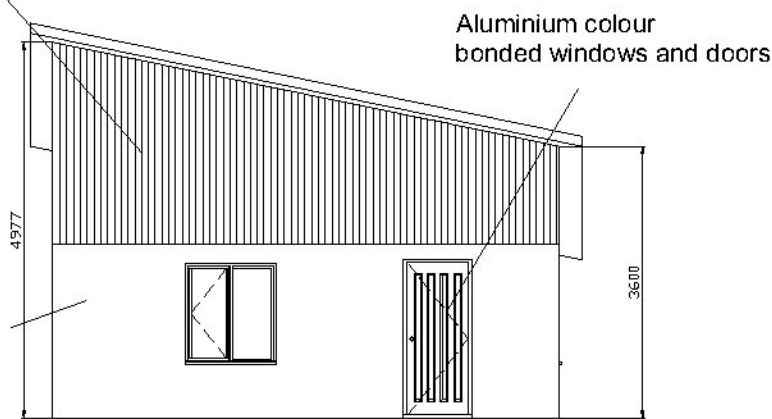
Proposed Garage NW Elevation
