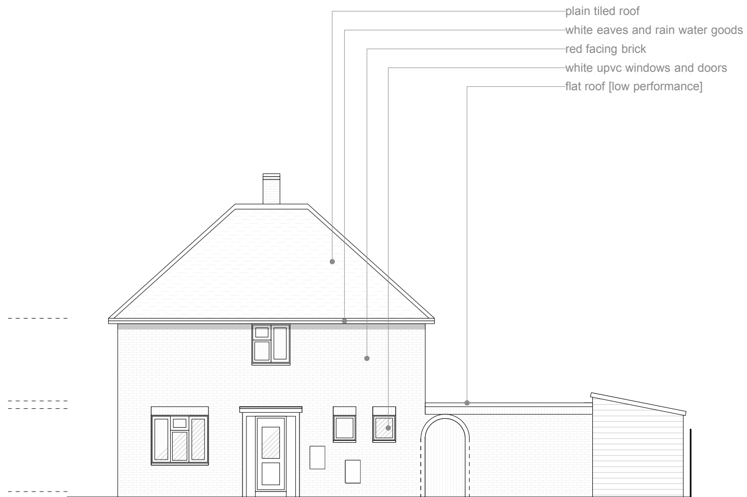
01 existing west elevation [Crittall Close] Scale: 1:100
