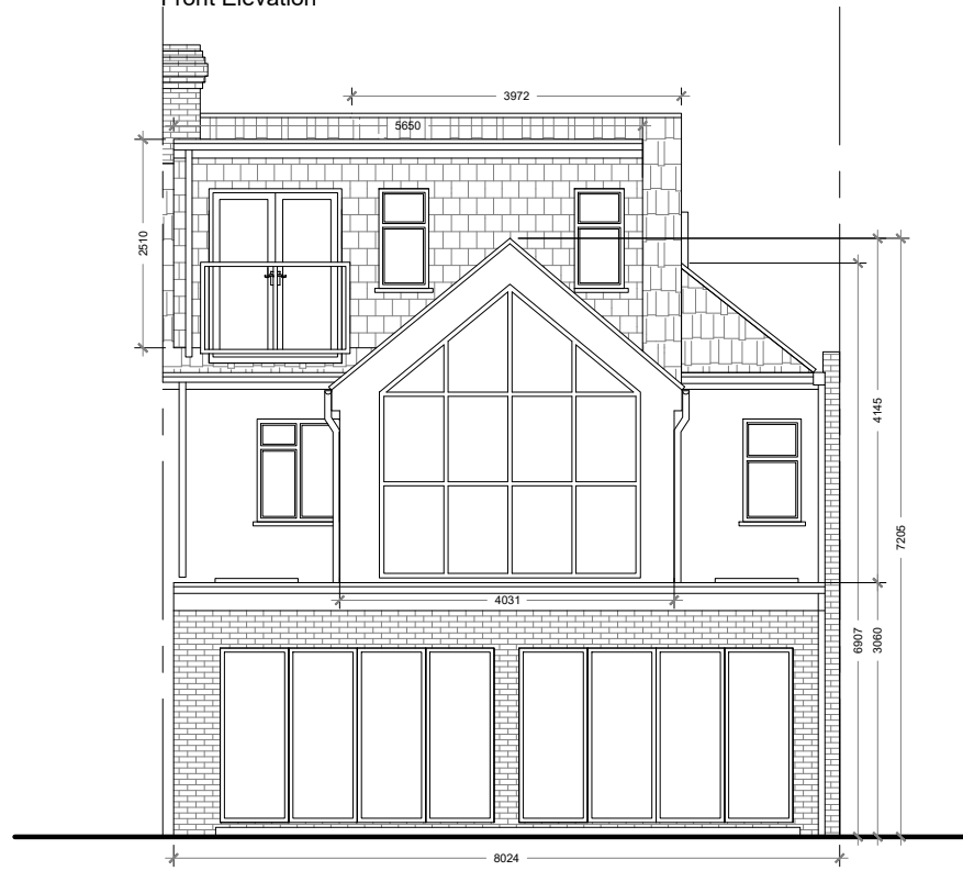
Rear Elevation
