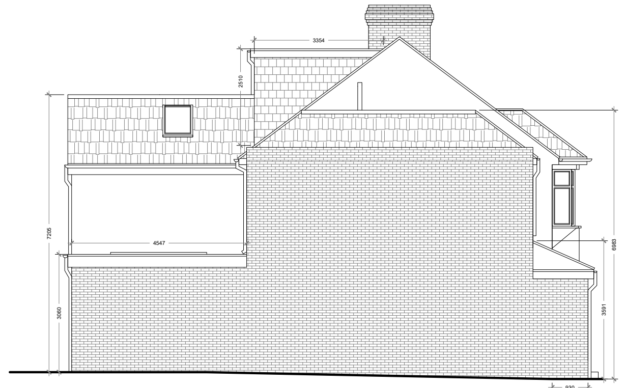
Side Elevation
