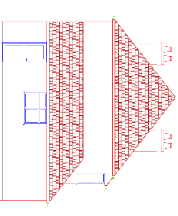
EXISTING LEFT SIDE VIEW
