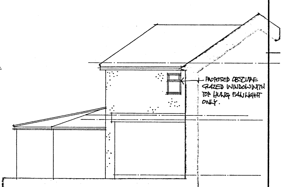
REAR FLANK
