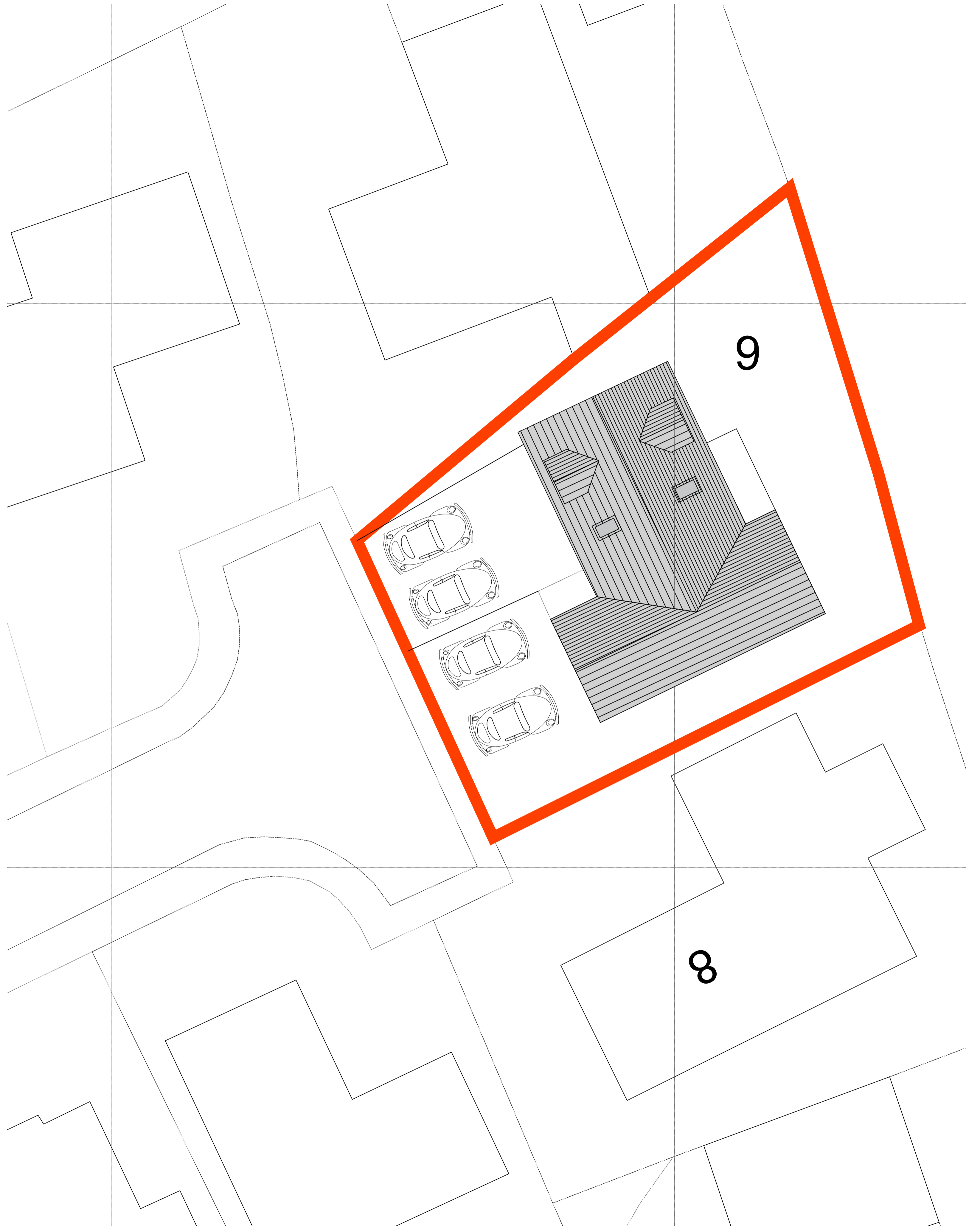
PROPOSED SITE BLOCK PLAN SCALE 1:100
