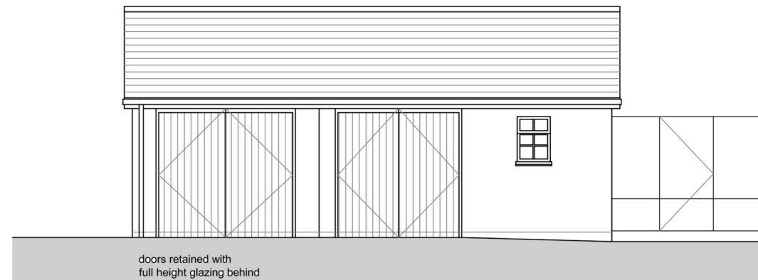
doors retained with full height glazing behind front elevation 1:100
