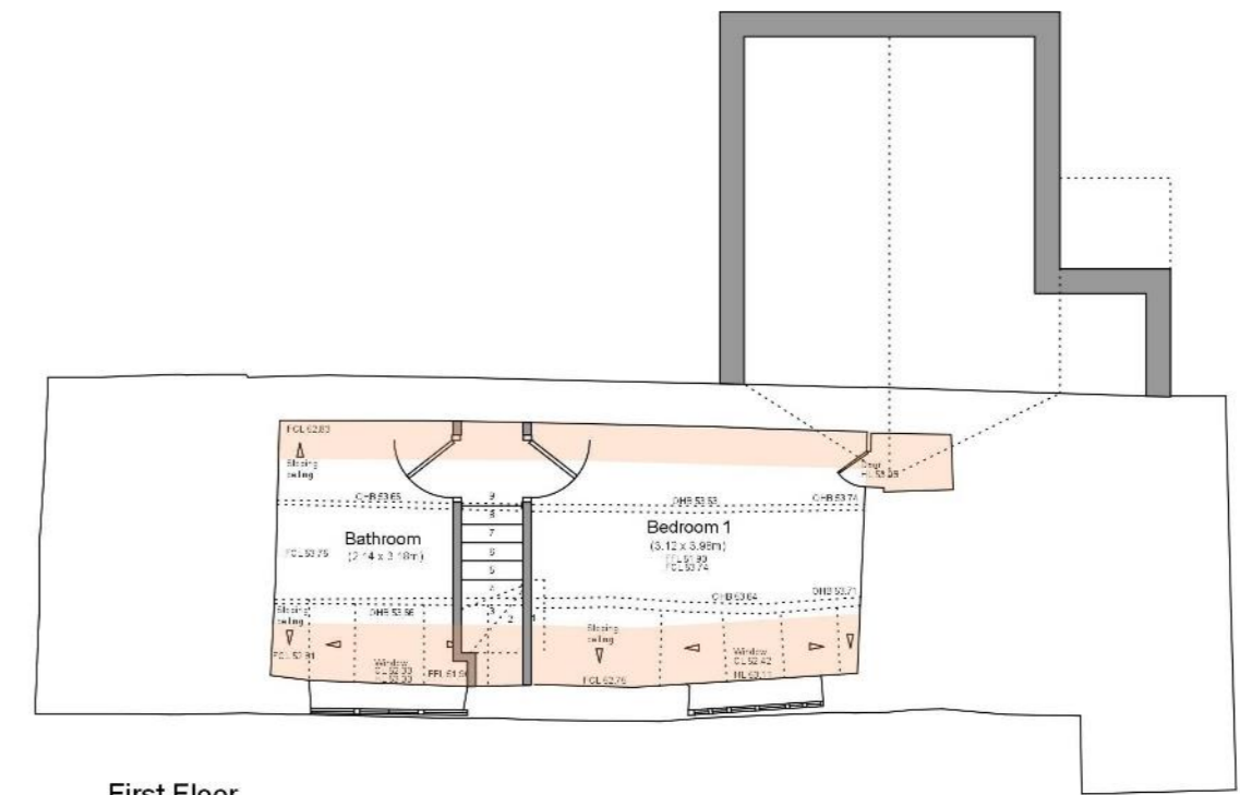
First Floor
