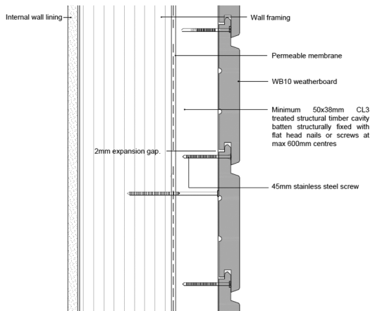
Fig 3 - WB10 Horizontal fixing detail
