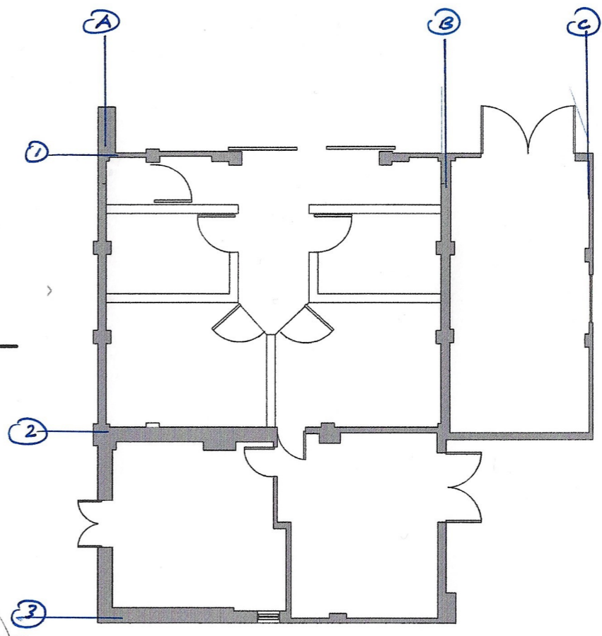
EXISTING PLAN @1:100
