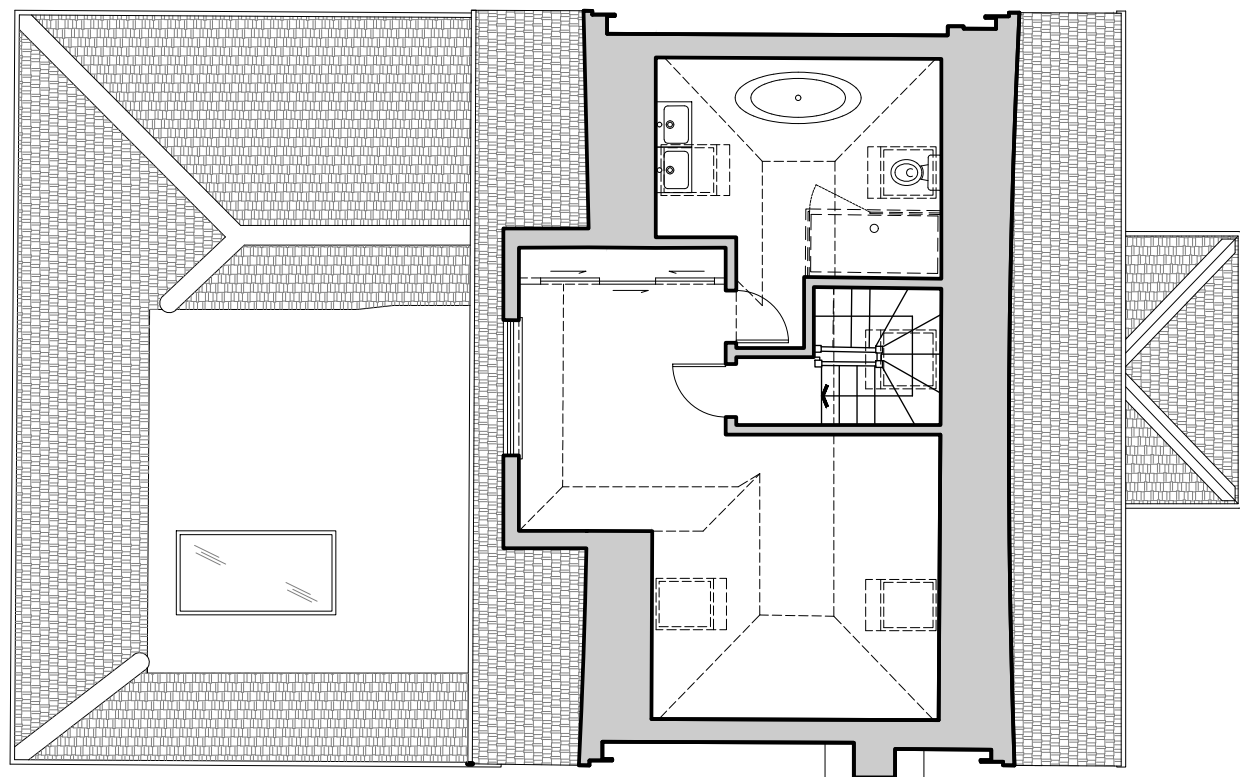
01 Existing Second Floor Plan E(02)_101 1:100@A3
