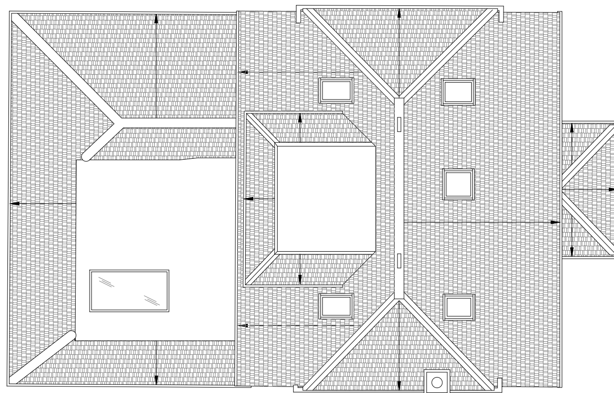
02 Existing Roof Plan E(02)_101 1:100@A3
