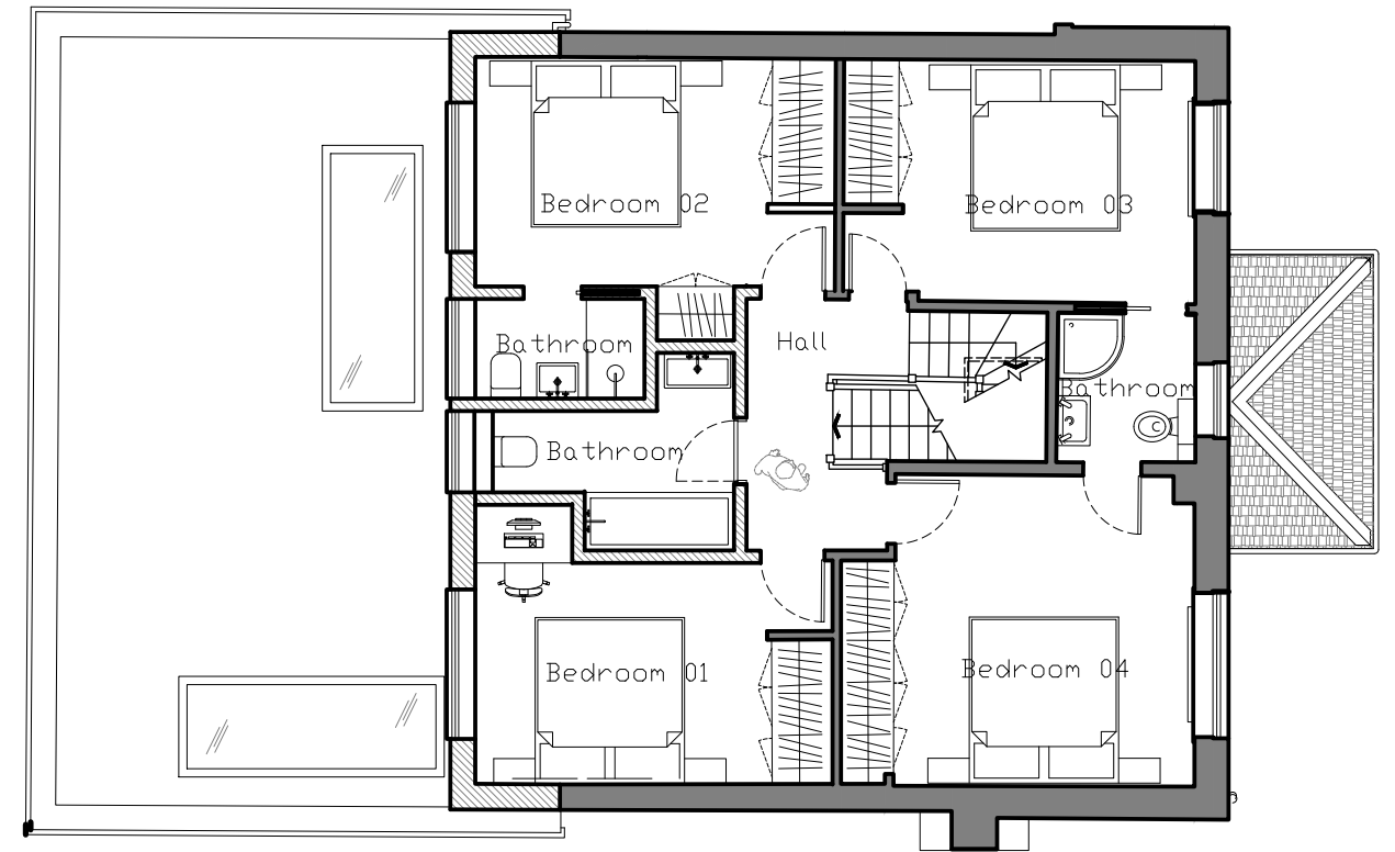
02 P(02)_100 Proposed First Floor Plan 1:100@A3
