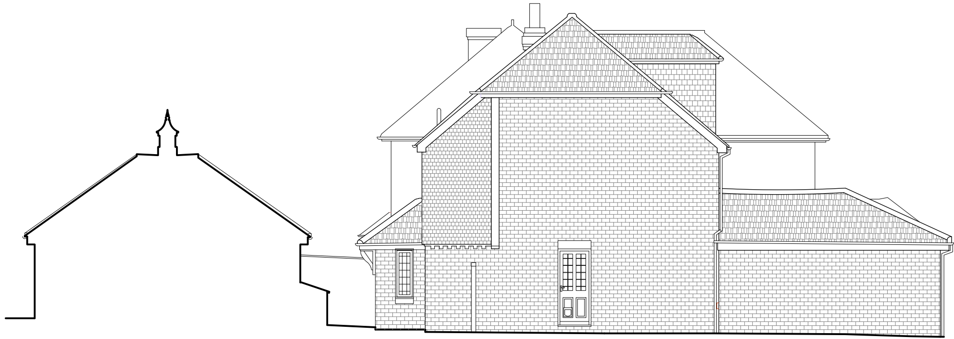
Side Elevation 01 1:100@A3
