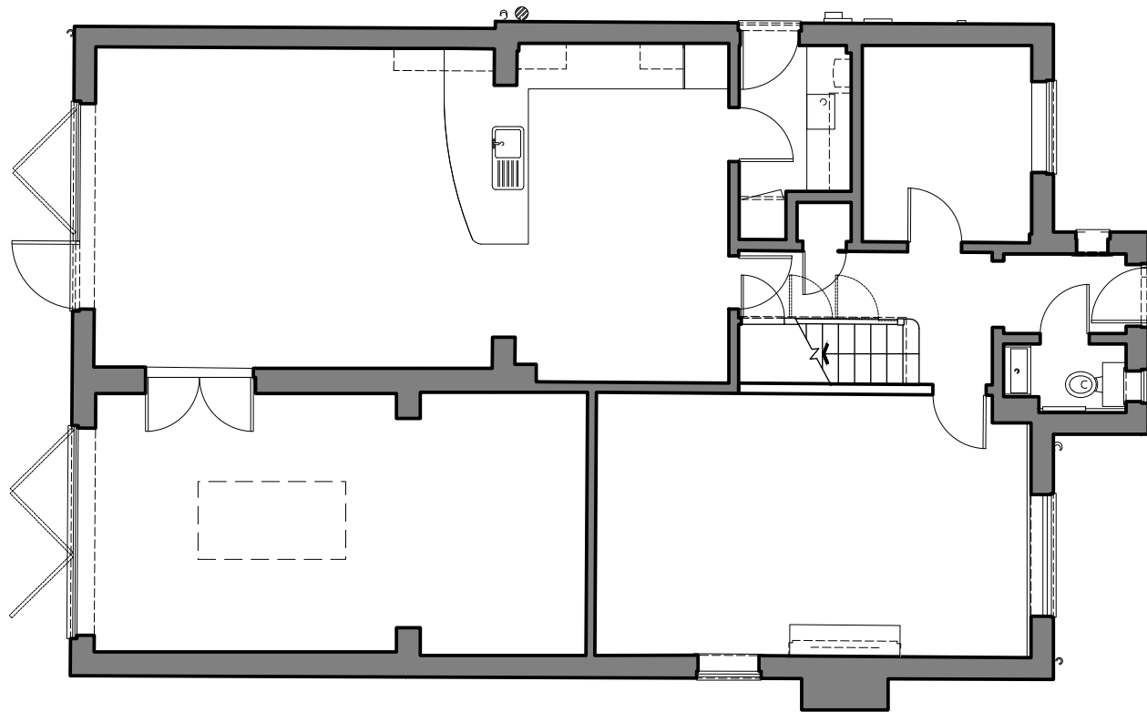
01 Existing Ground Floor Plan E(02)_100 1:100@A3
